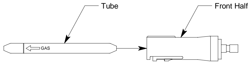
Figure 48: Inserting New Tube Into Front Half
